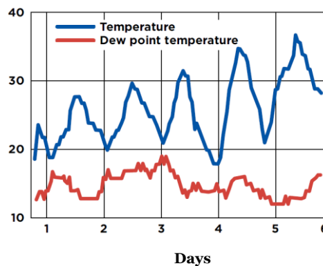
Transport with dew point control Dew point temperature is kept below surface temperature, preventing condensation and moisture damage.
