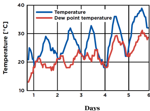
Transport without dew point control Condensation occurs when surface temperature and dew point temperature are equal.
